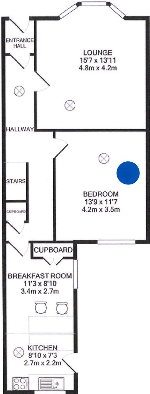
GROUND FLOOR APPROX. FLOOR AREA 668 SQ.FT. (62.1 SQ.M.)
